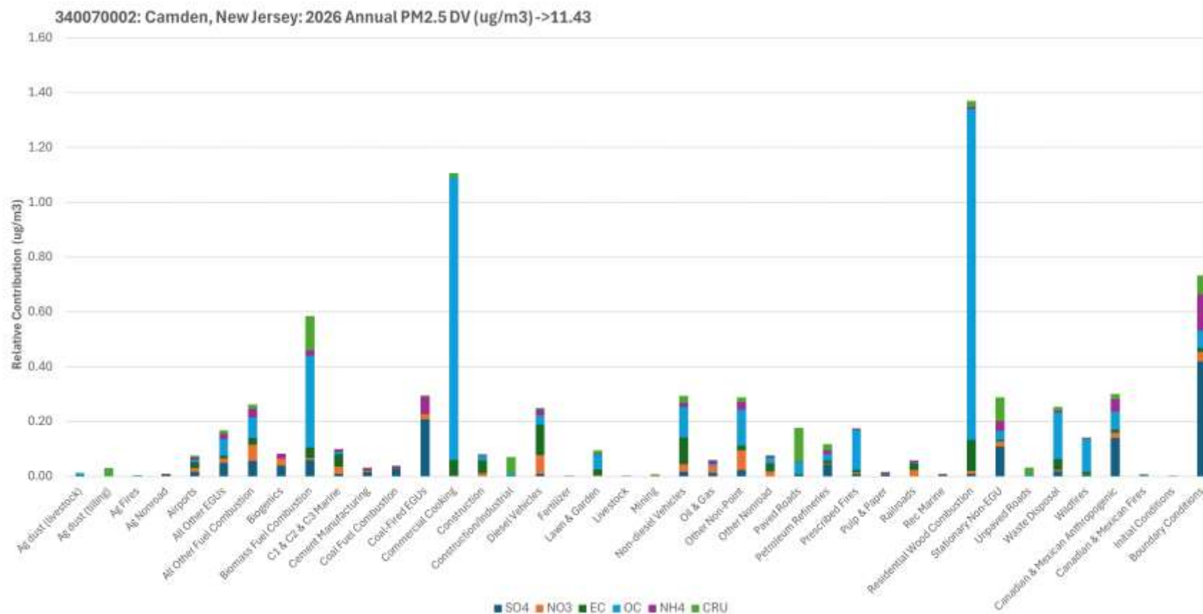
Figure 16. Stacked bar chart of category and traced species to modeled annual PM 2.5 design value at monitor 340070002.
