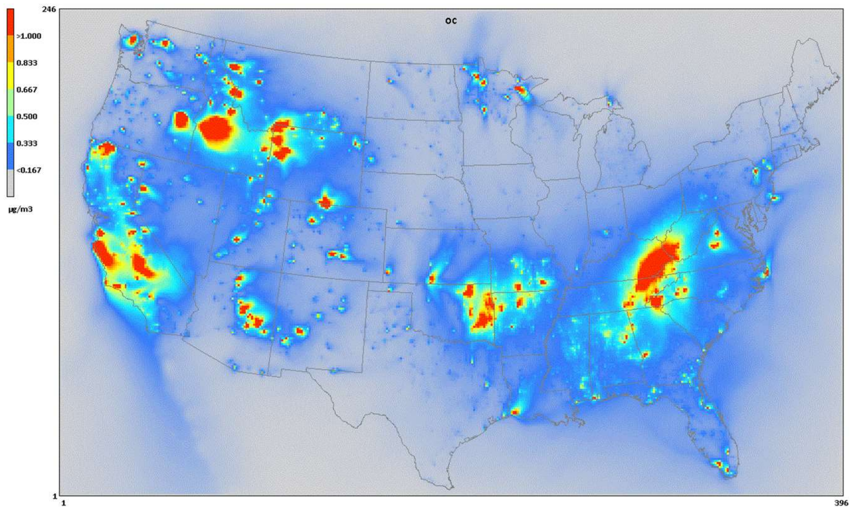
Figure 7. Modeled annual organic carbon concentrations ( \mu\text{g}/\text{m}^3 ) from 2026 base case simulation for wildfire category.
