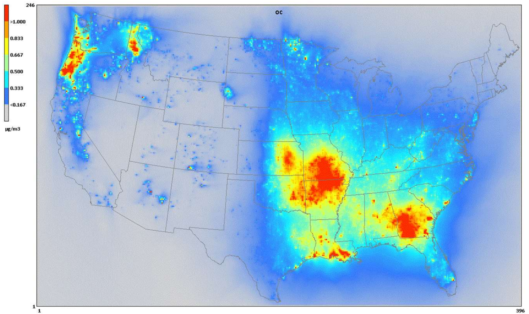
Figure 9. Modeled annual organic carbon concentrations ( \mu\text{g}/\text{m}^3 ) from 2026 base case simulation for prescribed fire category.
