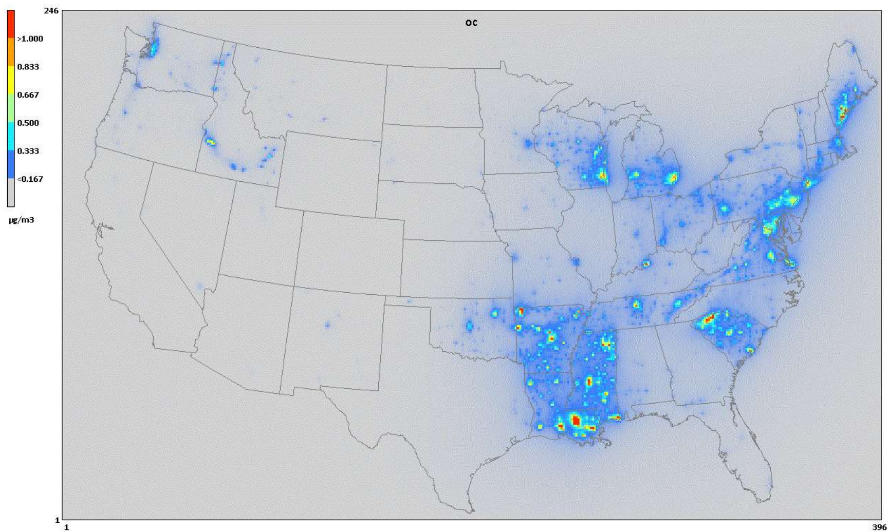
Figure 12. Modeled annual organic carbon concentrations ( \mu\text{g}/\text{m}^3 ) from 2026 base case simulation for biomass fuel combustion category.
