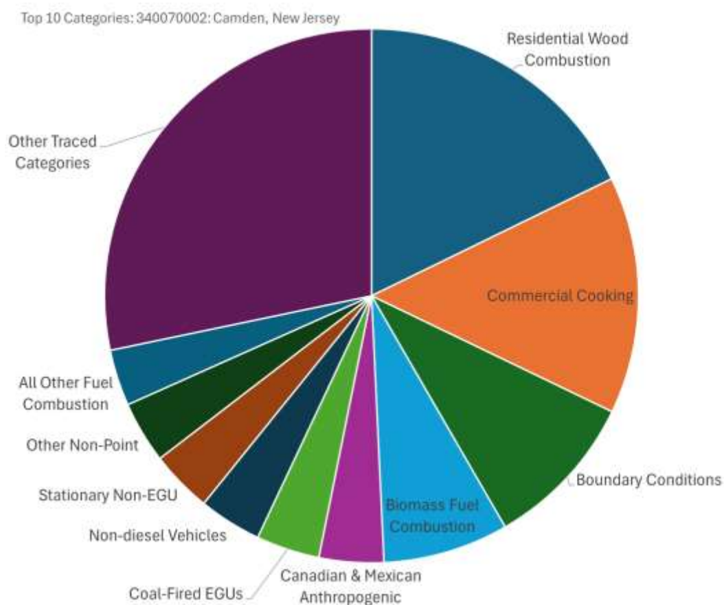
Figure 17. Pie chart of top 10 category contributions (and all other traced categories combined) at near-road monitor 340070002 in Camden County, New Jersey.
