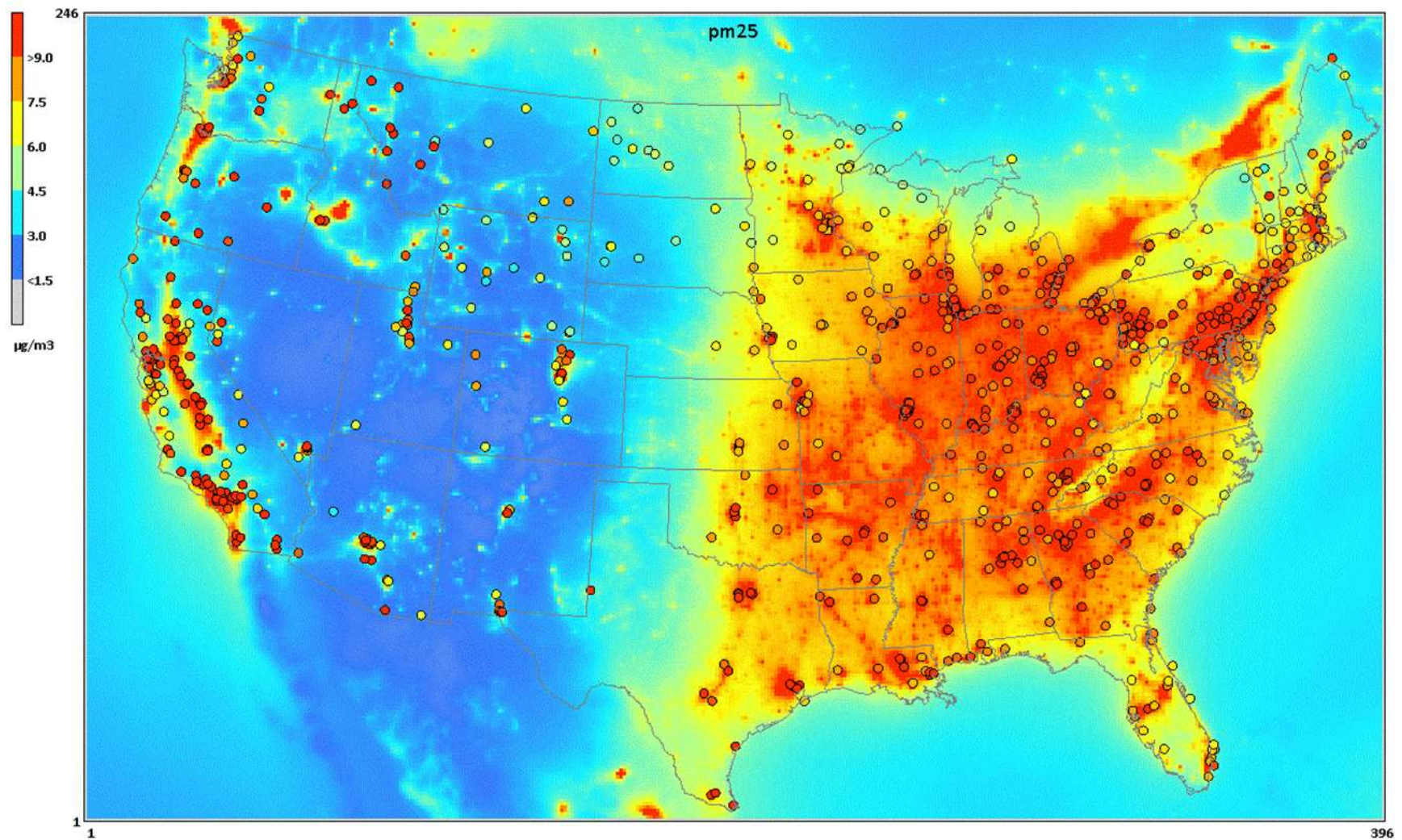
Figure 5. Modeled total annual PM 2.5 concentrations (µg/m³) from 2026 base case simulation.
