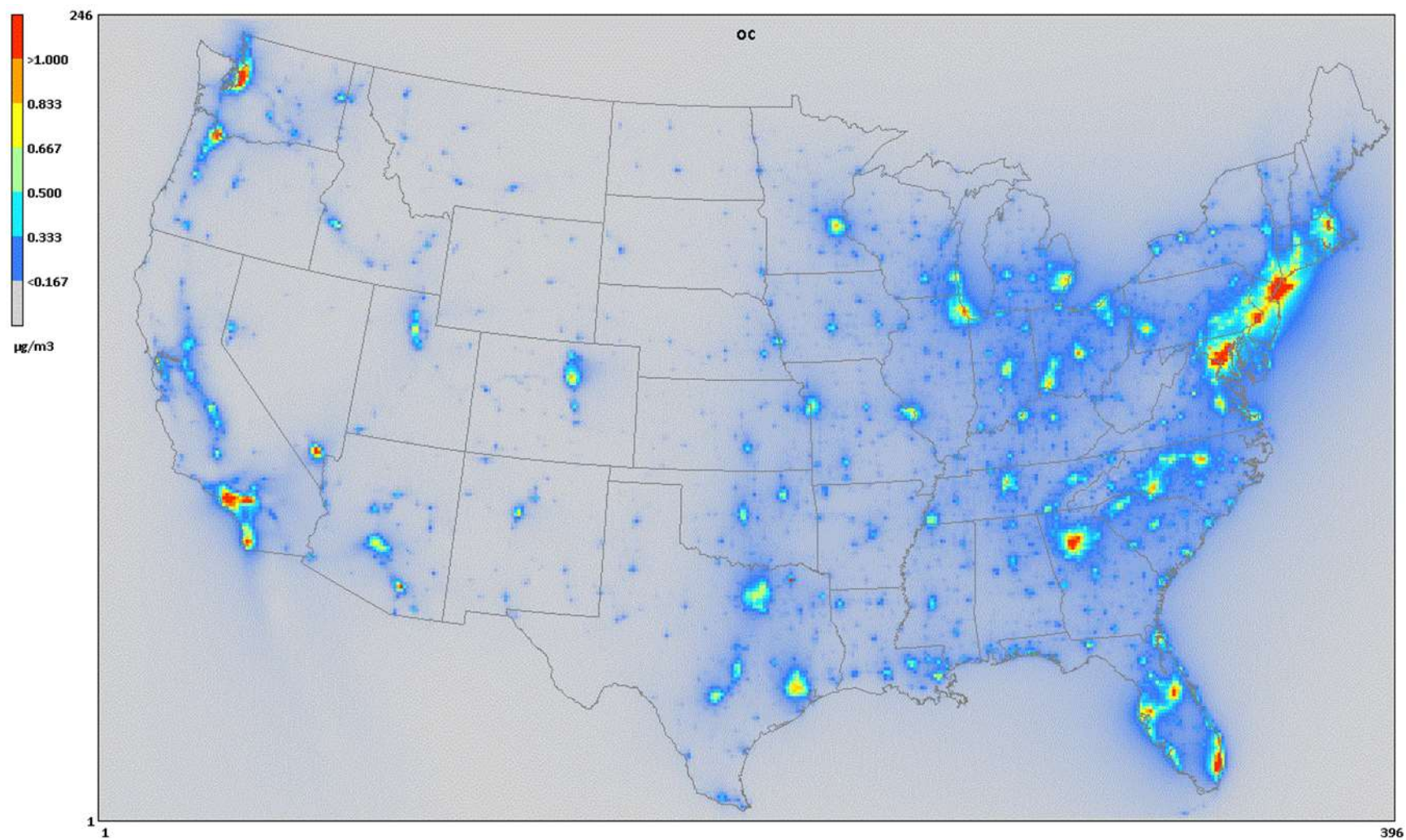
Figure 10. Modeled annual organic carbon concentrations ( \mu\text{g}/\text{m}^3 ) from 2026 base case simulation for commercial cooking category.
