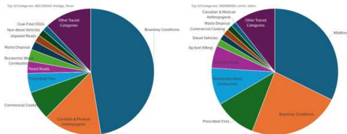
Figure 18. Pie charts of top 10 category contributions (and all other traced categories combined) at border monitor 482150043 in Hidalgo County, Texas (left) and at small mountain monitor 160590004 in Lemhi County, Idaho (right).
