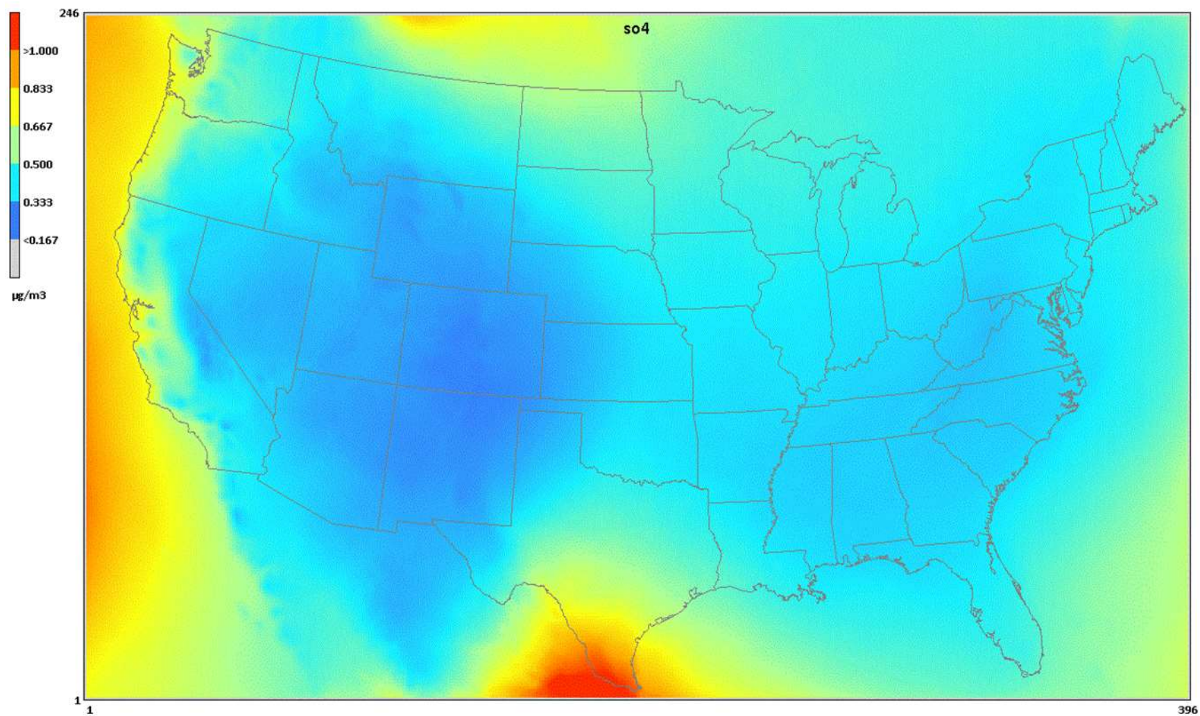
Figure 6. Modeled annual particulate sulfate concentrations ( \mu\text{g}/\text{m}^3 ) from 2026 base case simulation for boundary condition category.
