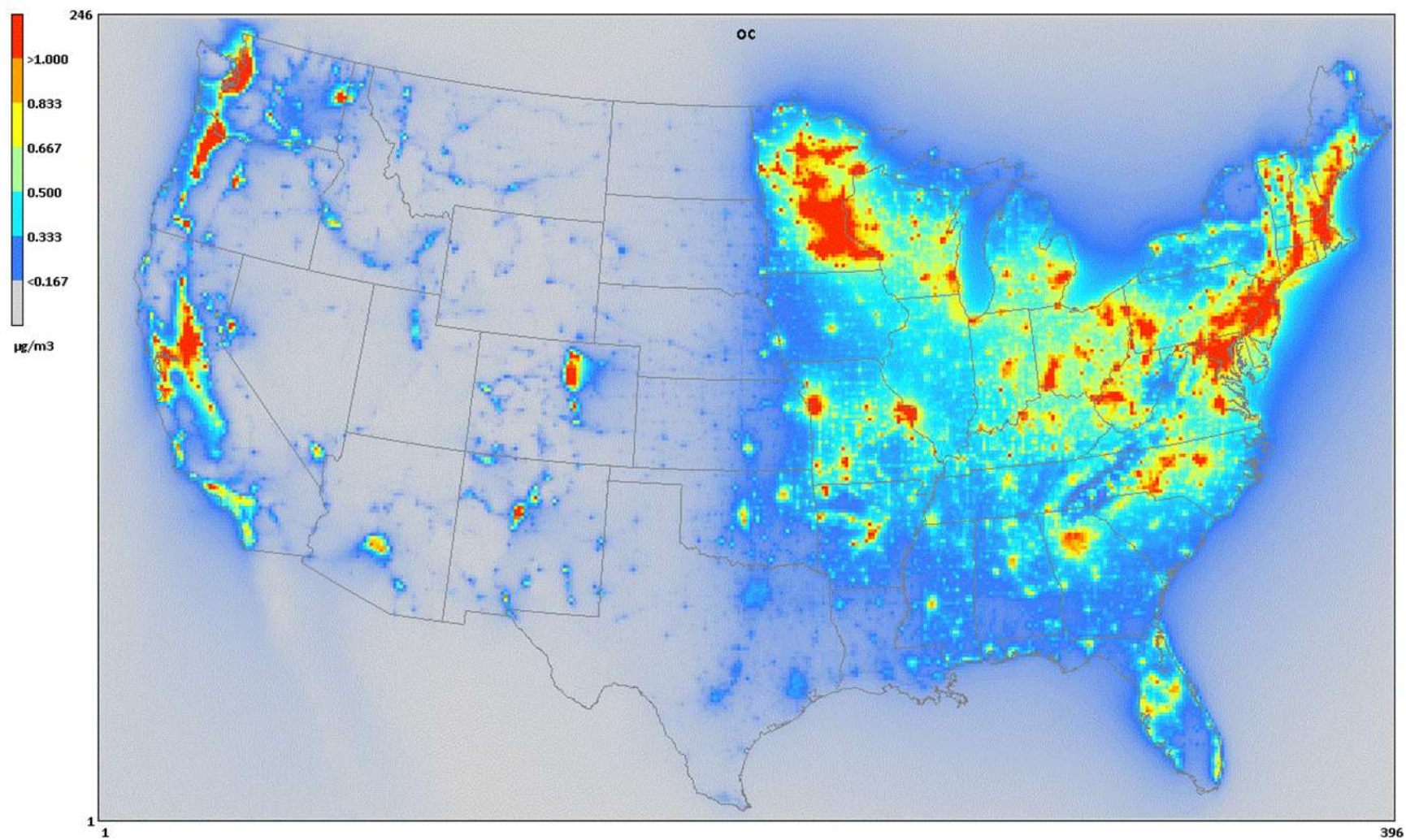
Figure 8. Modeled annual organic carbon concentrations ( \mu\text{g}/\text{m}^3 ) from 2026 base case simulation for residential wood combustion category.
