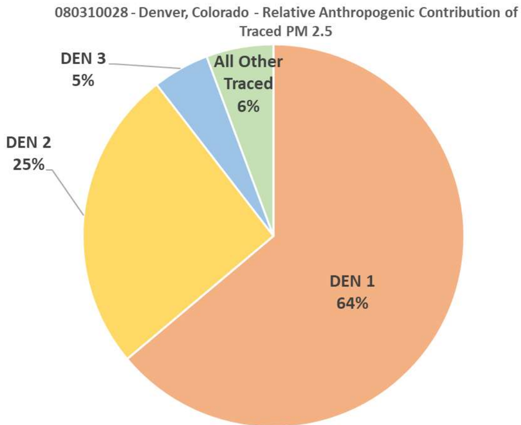
Figure 23. Relative contribution by region to Denver, CO monitor 080310028.
