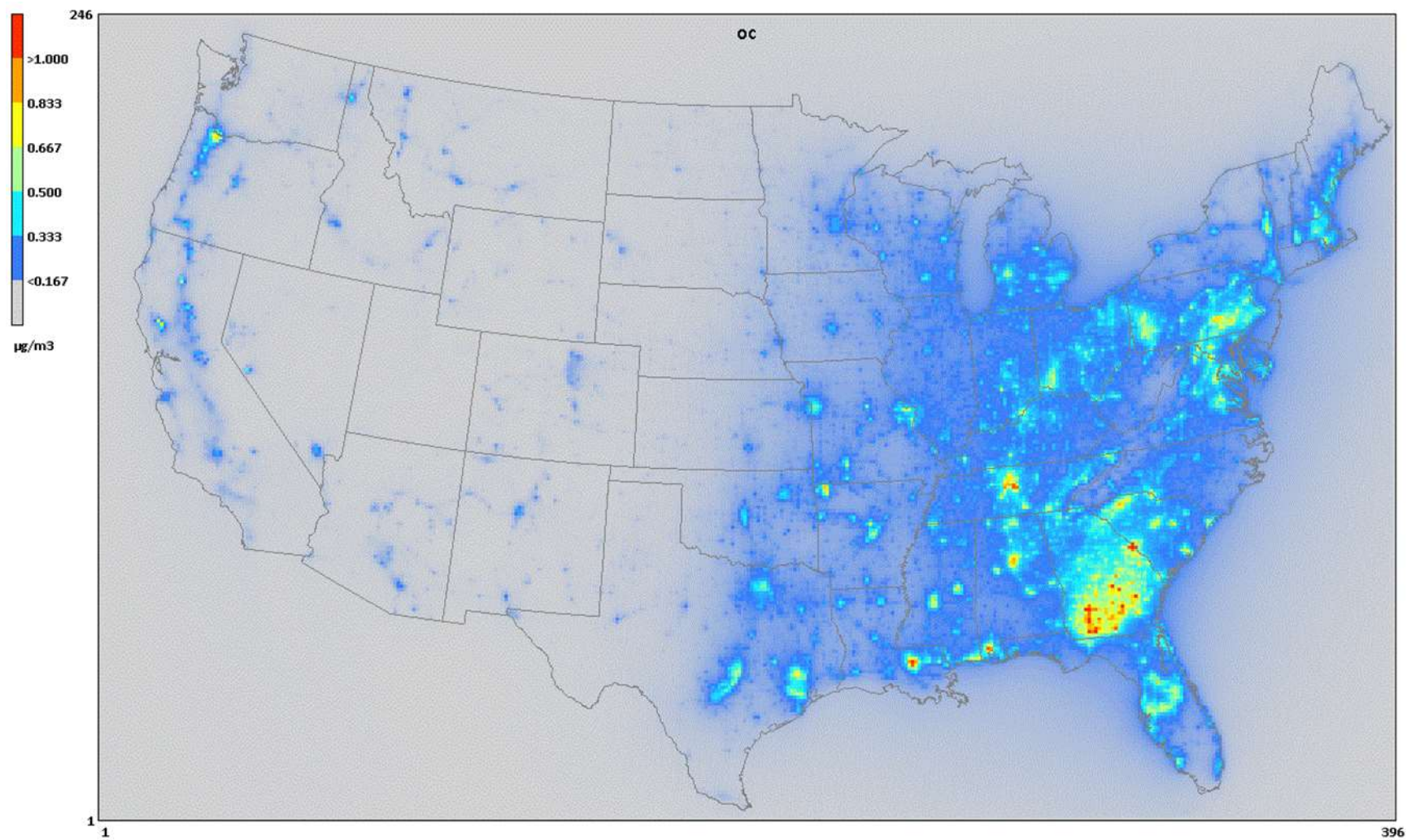
Figure 14. Modeled annual organic carbon concentrations ( \mu\text{g}/\text{m}^3 ) from 2026 base case simulation for waste disposal category.
