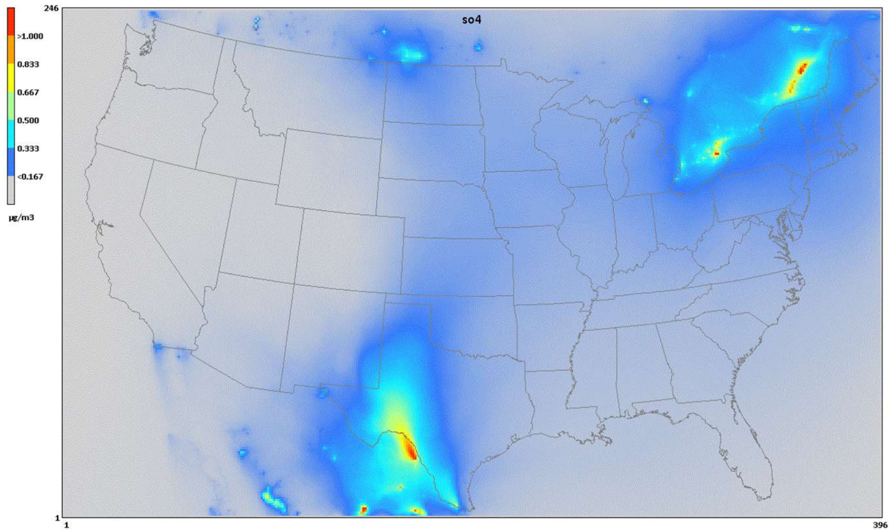
Figure 11. Modeled annual particulate sulfate concentrations ( \mu\text{g}/\text{m}^3 ) from 2026 base case simulation for Canadian and Mexican anthropogenic category.
