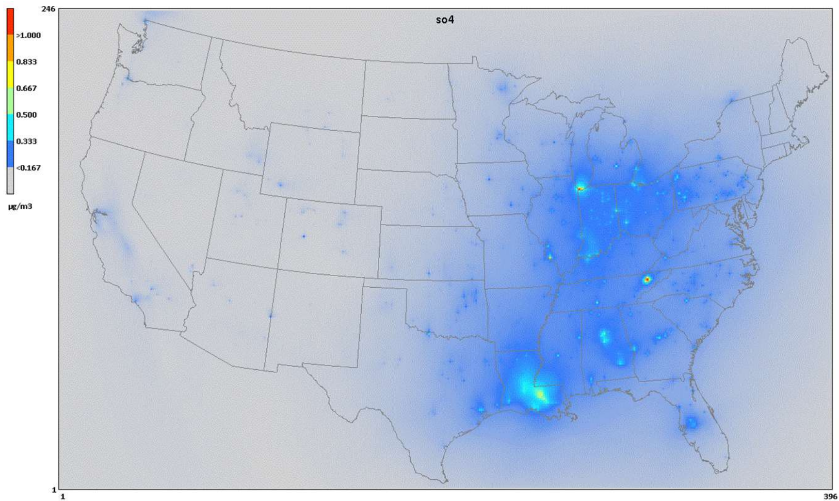
Figure 13. Modeled annual primary sulfate concentrations ( \mu\text{g}/\text{m}^3 ) from 2026 base case simulation for stationary non-EGU category.
