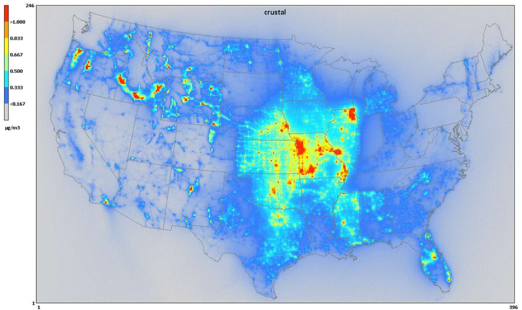
Figure 15. Modeled annual crustal mass concentrations (µg/m³) from 2026 base case simulation for unpaved roads category.
